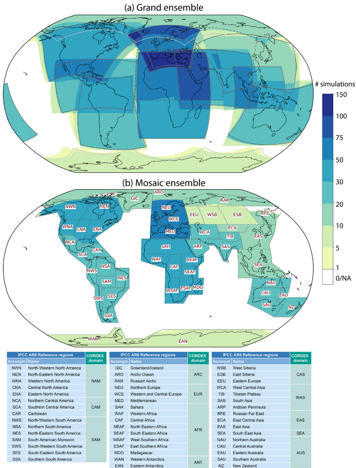
Fig. 1. Number of historical simulations available from the worldwide C3S CORDEX dataset for (a) the multidomain grand ensemble and (b) the single-domain mosaic ensemble. Gray lines in (a) correspond to the boundaries of the 14 CORDEX domains (see Table 2), which are exceeded in many cases by the actual simulation domains. Gray lines in (b) correspond to the IPCC AR6 WGI reference regions (Iturbide et al. 2020) which are used to create the mosaic [note that CORDEX domains assigned to each region are shown in the table below, following Gutiérrez et al. (2021a) but including the CAS domain for EEU, WSB, and ESB regions]. Note that MED- and MENA-CORDEX domains are not used in the mosaics because they are overlapped by other domains with a higher number of simulations.
