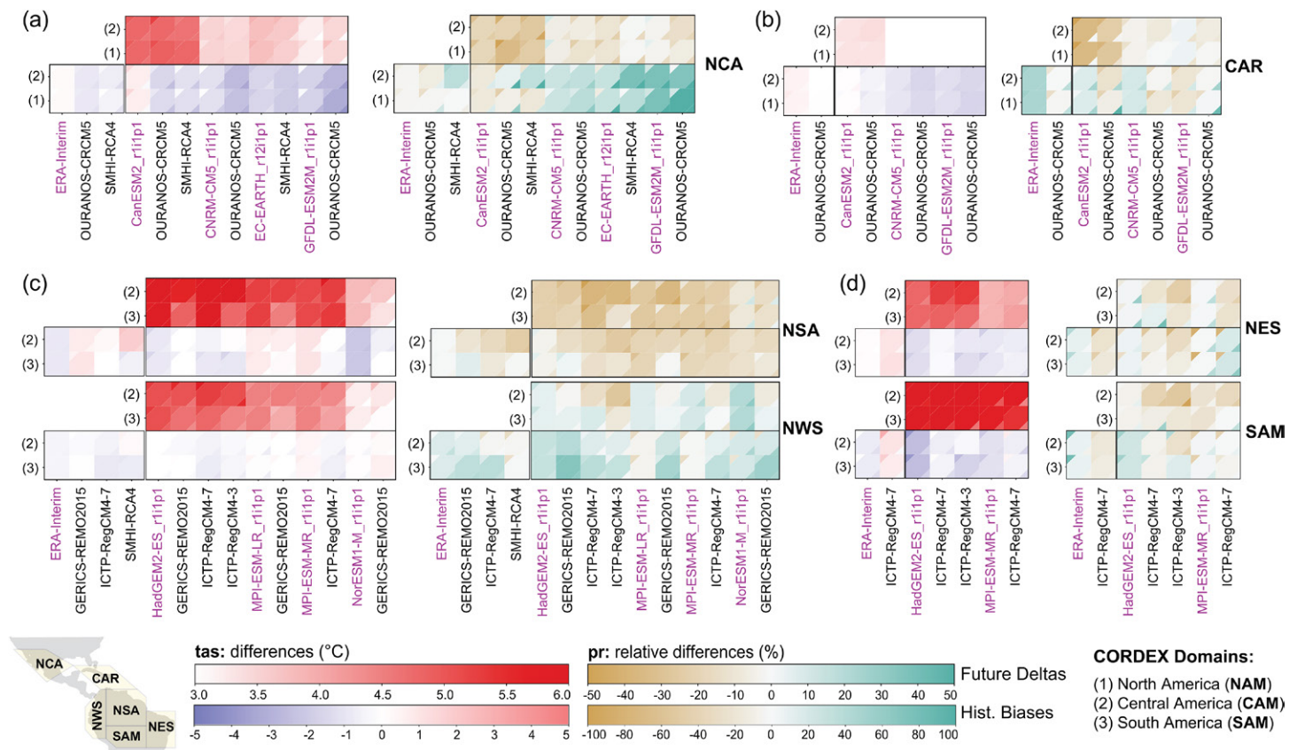
Fig. 4. Biases and future delta changes of regional overlaps for the American regions: (a) northern Central America (NCA), (b) Caribbean (CAR), (c) northern South America (NSA) and northwestern South America (NWS), and (d) northeastern South America (NES) and South American monsoon (SAM). Labels indicate the reference regions used in the IPCC AR6 (see Fig. 1b). Numbers in parenthesis indicate CORDEX domains. Columns correspond to the models (driving model labels highlighted in magenta followed by the RCMs nested into that model, in black text). The panels intercompare the biases (bottom) and the climate signals (top) for the different CORDEX domains providing simulations for the same geographical regions. Colored cells show the biases or climate change signals considering the whole year (central color), the boreal summer months (JJA, upper-left corner), and the boreal winter months (DJF, lower-right corner).
